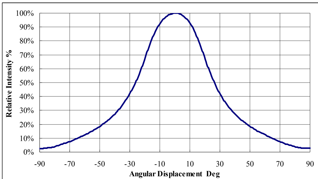
Fig. Typical Representative Spatial Radiation Pattern : 60 degree
