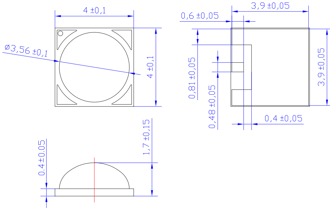
Fig. Package Outline Drawing.
