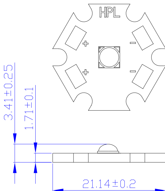
Fig. Assembly Outline Drawing.
