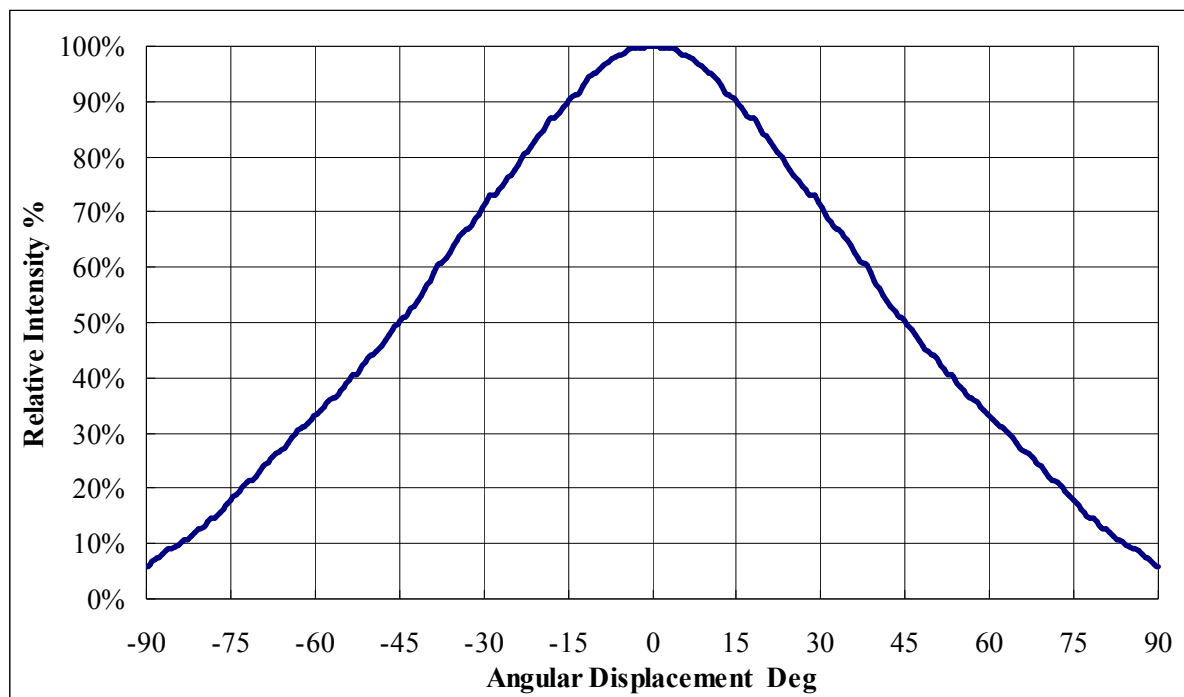
Fig. Typical Representative Spatial Radiation Pattern : 90 degree
